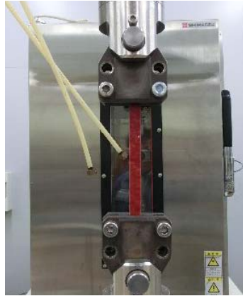
Figure 11. Setup of Level-2 cyclic strain test
