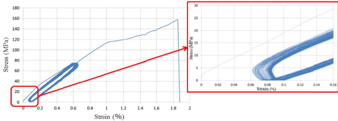
Figure 9. Record of cyclic strain test
