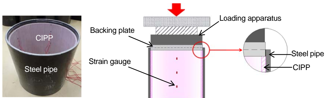
Figure 5. Test setup
